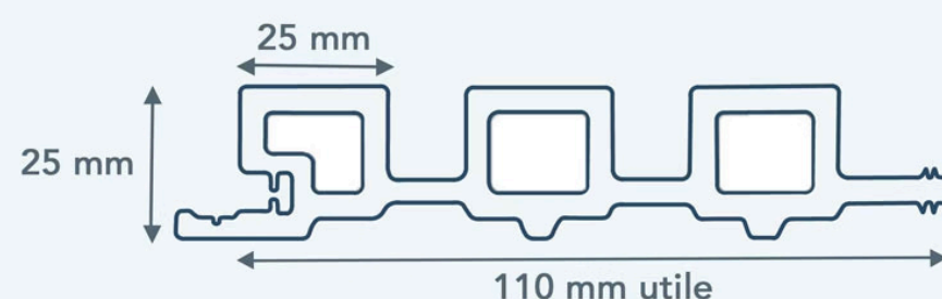
PROFIL XS EN CARRÉ ULTRAPROTECT
